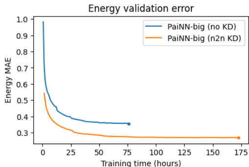
Figure 2. Energy validation error of PaiNN without (blue) and with (orange) knowledge distillation from GemNet-OC, trained for the same number of steps (1 million). Validation on a random sample of size 30k samples from the in-distribution OC20 validation set.
